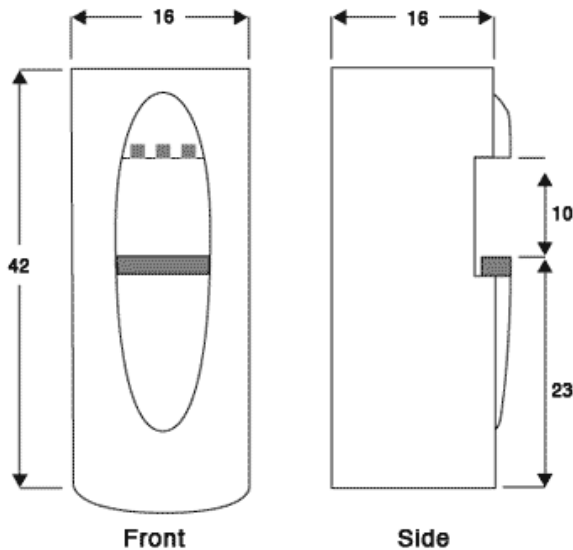
PWC-3500 Dimensions (inches)
